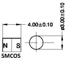
SMCO5
